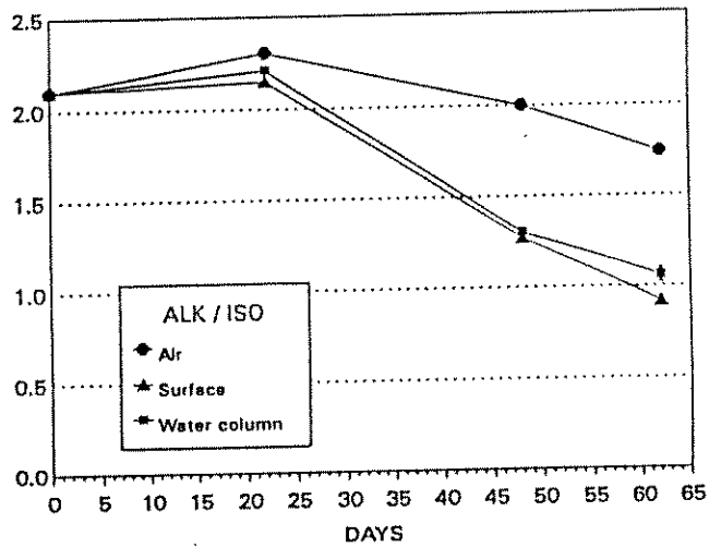
Fig.11 Winter (long-term) experiment: biodegradation of crude oil at different immersion levels (oil adsorbed on cotton strips).
