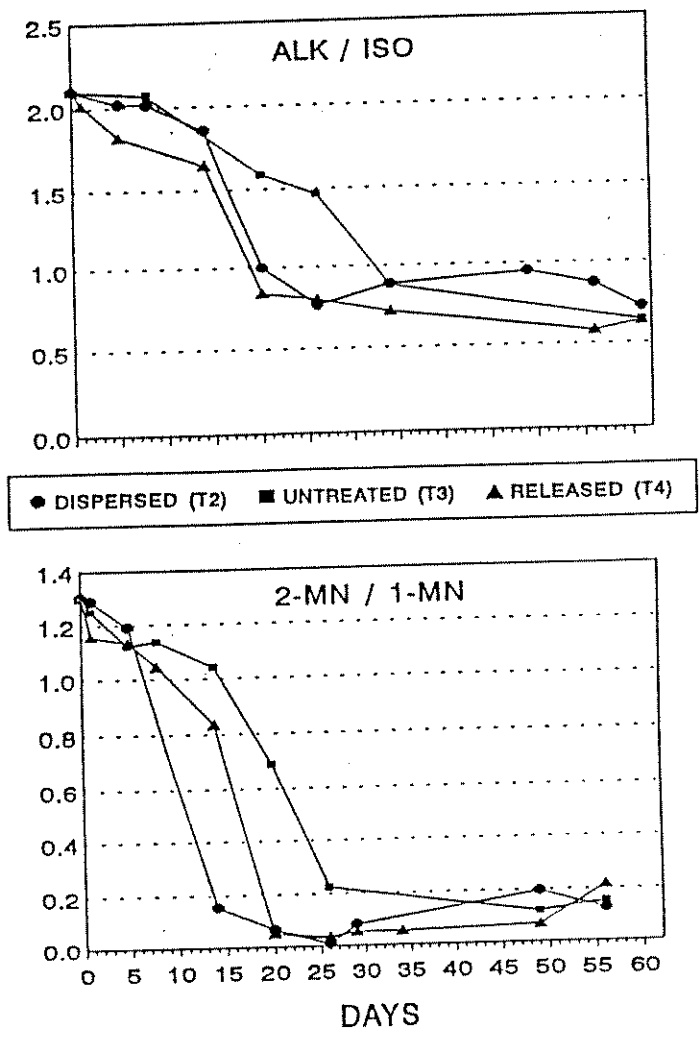
Fig.8 Winter (long-term) experiment: oil biodegradation with various oil treatments. (See Material & Methods for hydrocarbon ratios).
