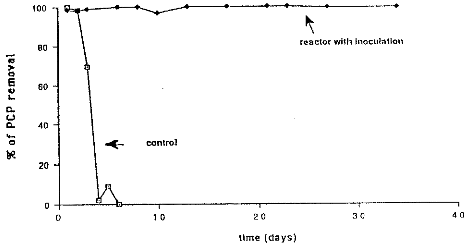
Fig 3: Percent removal of PCP in fluidized bed bioreactors.
