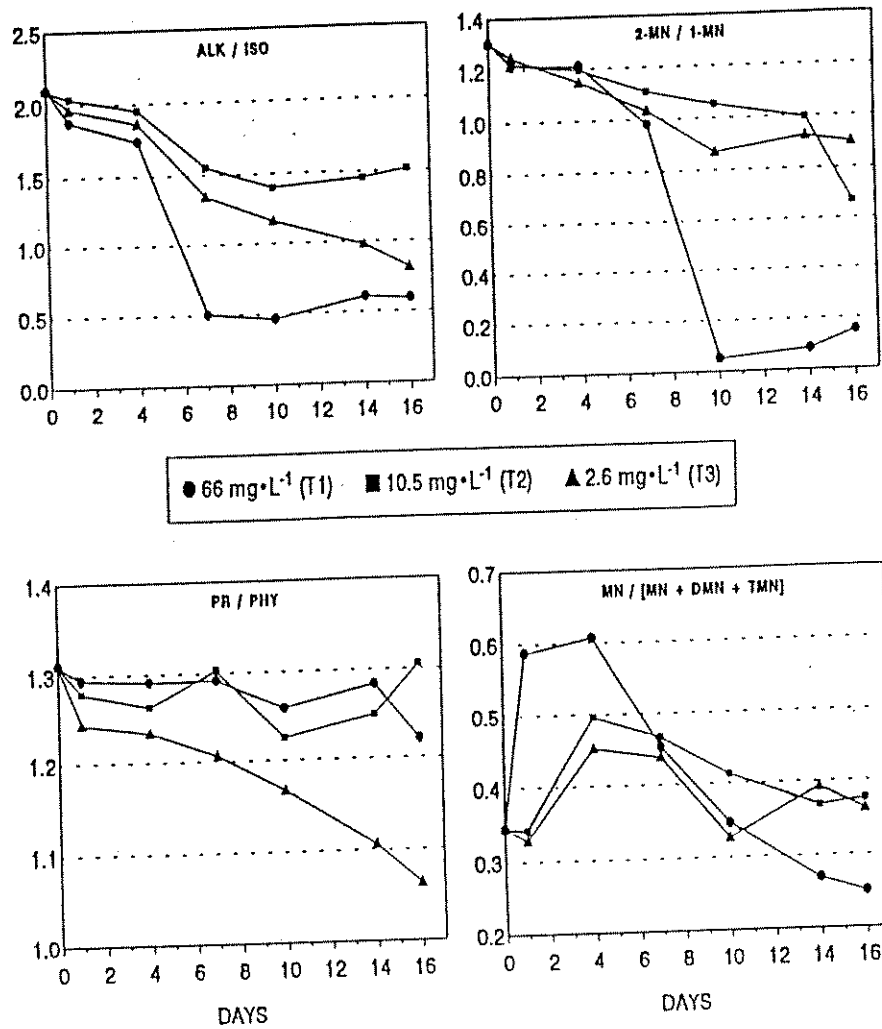
Fig.6 Spring experiment: oil biodegradation in tanks contaminated with various concentrations of dispersed oil (See Material & Methods for hydrocarbon ratios).
