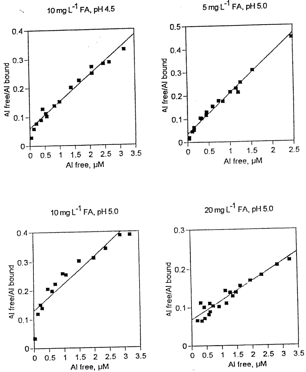
Figure 2. Langmuir isotherms determined from titration data with fulvic acid (FA).
